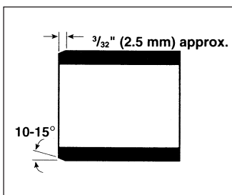
A 15° chamfer cut to a depth of approx. \frac{3}{32} ."
